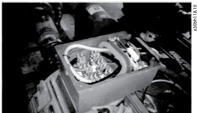
Illustration 5: Mounting of CM Cores Inside the Motor Terminal Box
