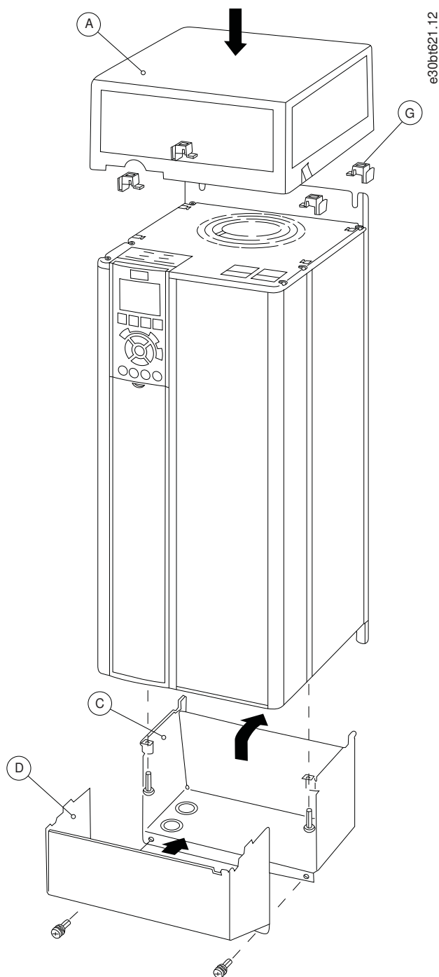
Illustration 22: IP21/UL Type 1 Kit on B4/C3/C4 Enclosure
