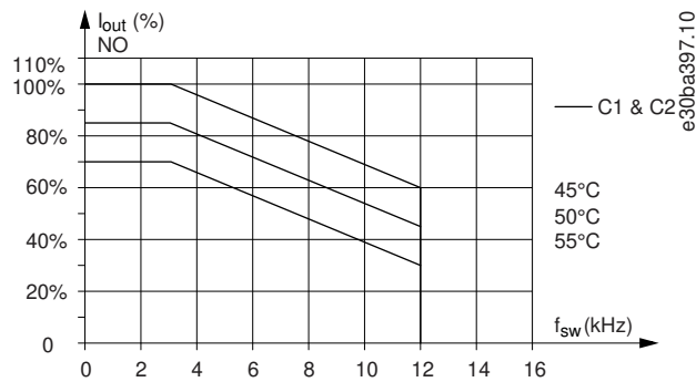
Illustration 52: Derating of I_{out} for Different T_{AMB,MAX} for Enclosures Sizes C1 and C2, using 60° AVM
