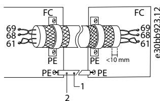
Illustration 65: Twisted-pair Cables
