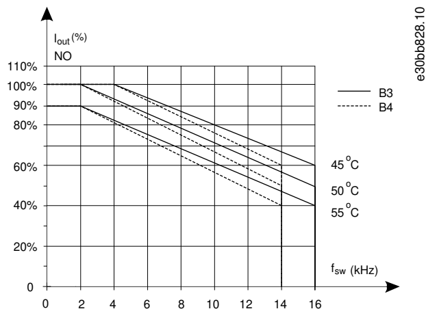
Illustration 46: Derating of I_{out} for Different T_{AMB,MAX} for Enclosure Sizes B3 and B4, using 60° AVM
