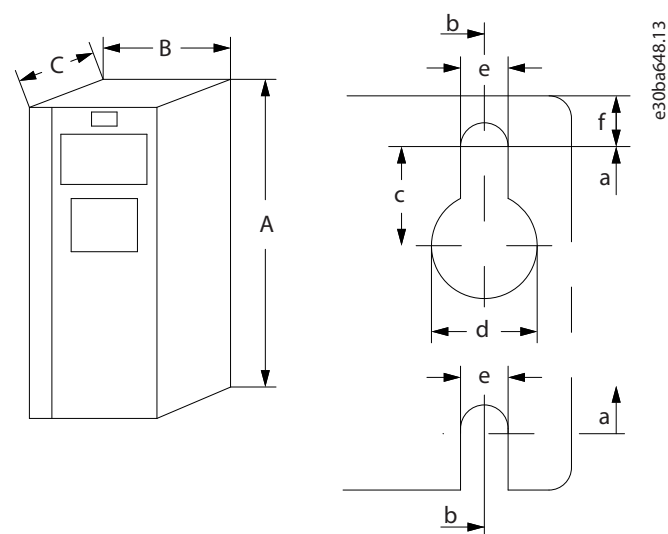
Illustration 30: Top and Bottom Mounting Holes
