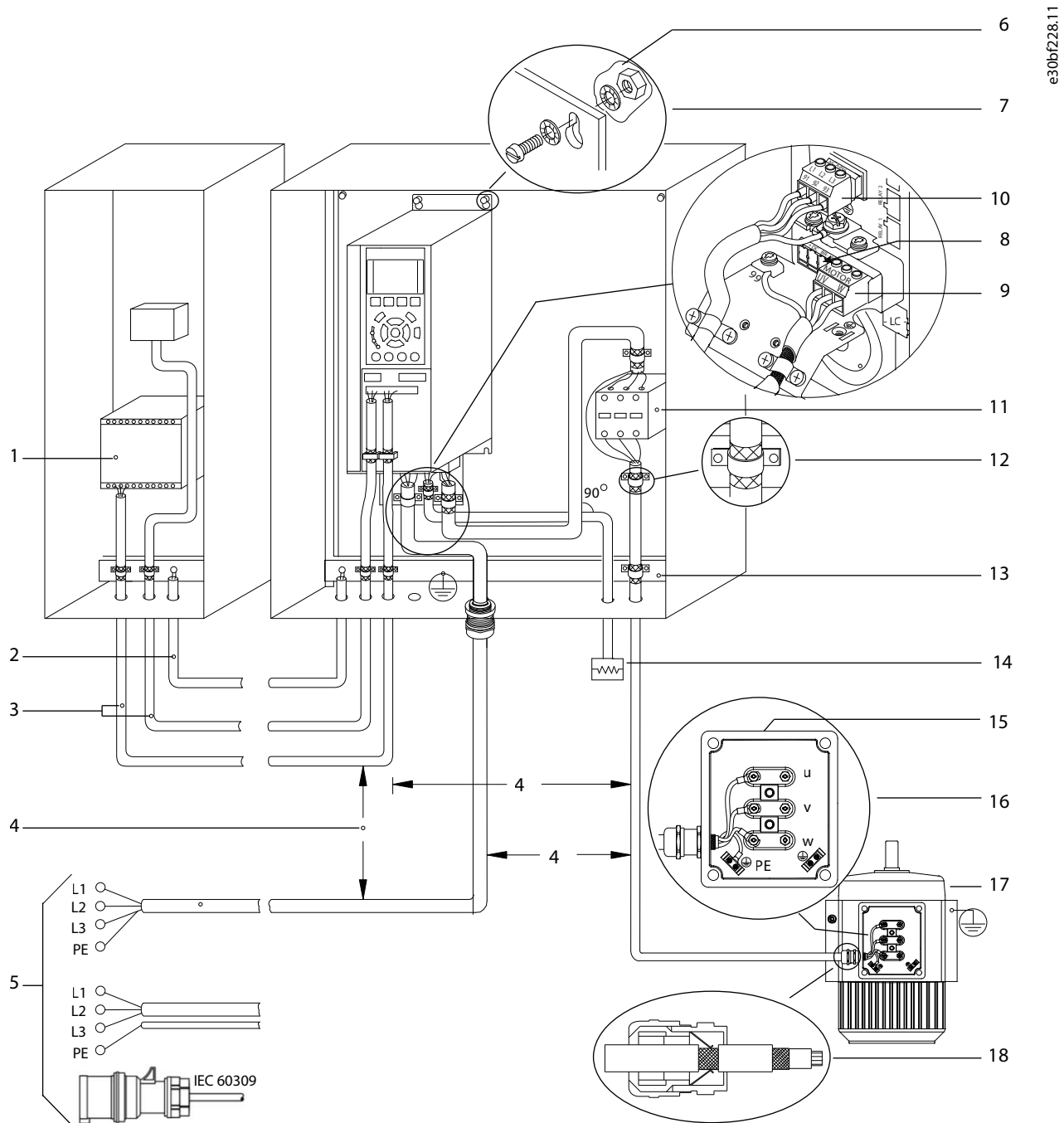
Illustration 61: EMC-compliant Electrical Connection
