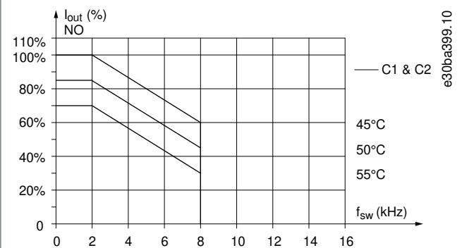
Illustration 53: Derating of I_{out} for Different T_{AMB,MAX} for Enclosures Sizes C1 and C2, using SFAVM
