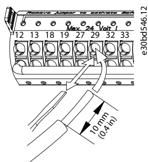
Illustration 67: Connecting Control Wires
