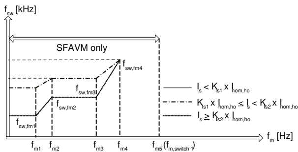
Illustration 16: Switching Frequency ( f_{sw} ) Variation for Different Stator Frequencies ( f_m )
