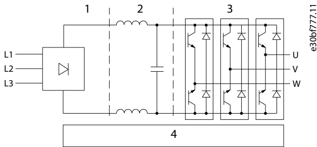
Illustration 87: Internal Processing
