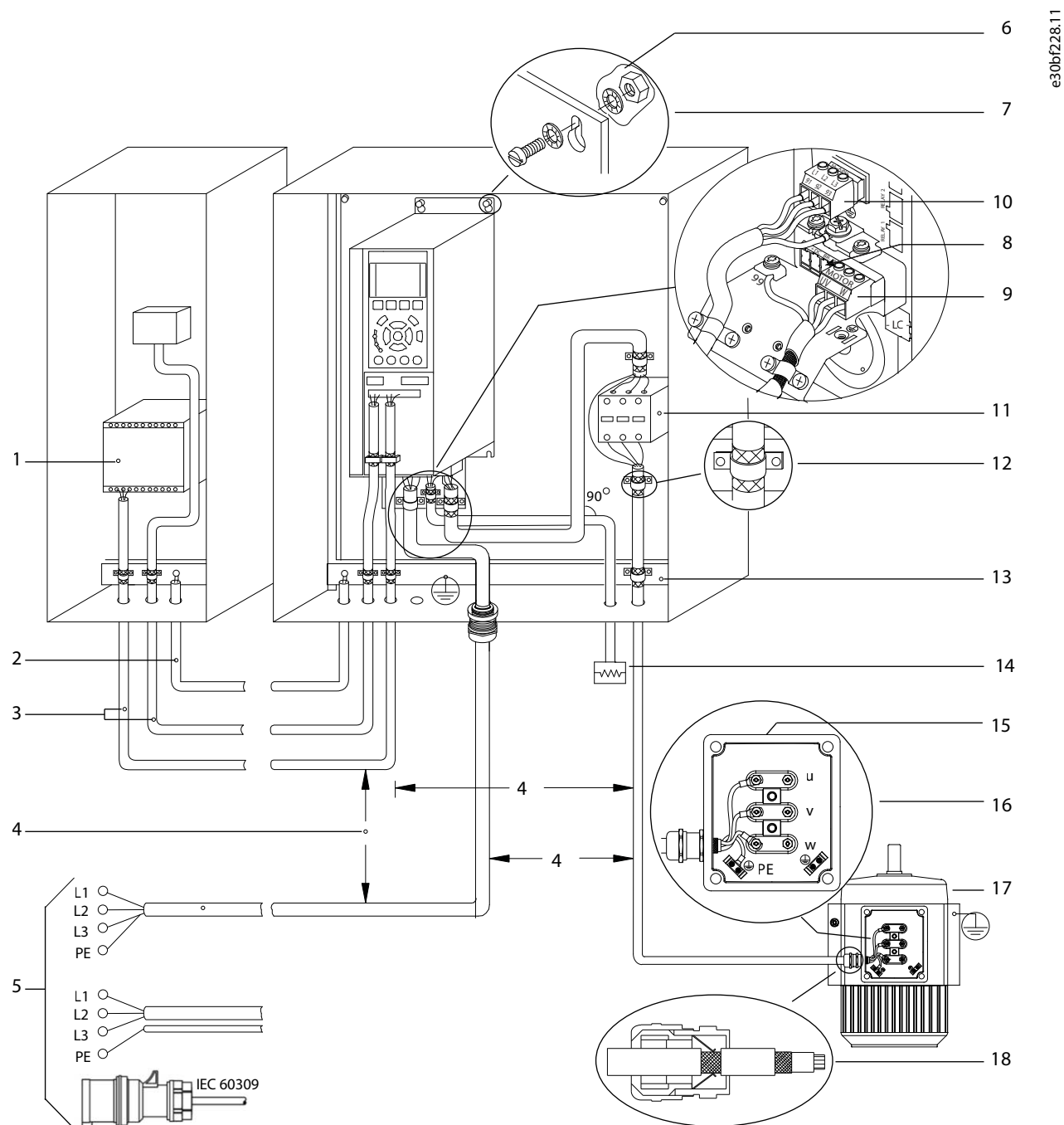
Illustration 82: Example of Proper EMC Installation
