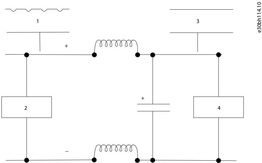
Illustration 9: Wiring Diagram of the DC Link
