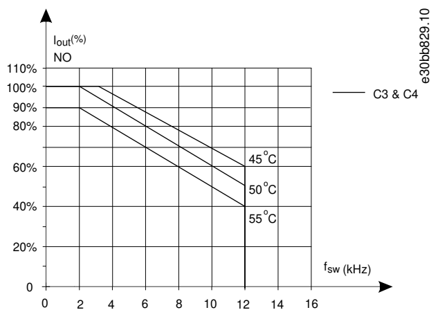
Illustration 54: Derating of I_{out} for Different T_{AMB,MAX} for Enclosures Sizes C3 and C4, using 60° AVM
