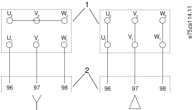
Illustration 86: Motor Cable Connection
