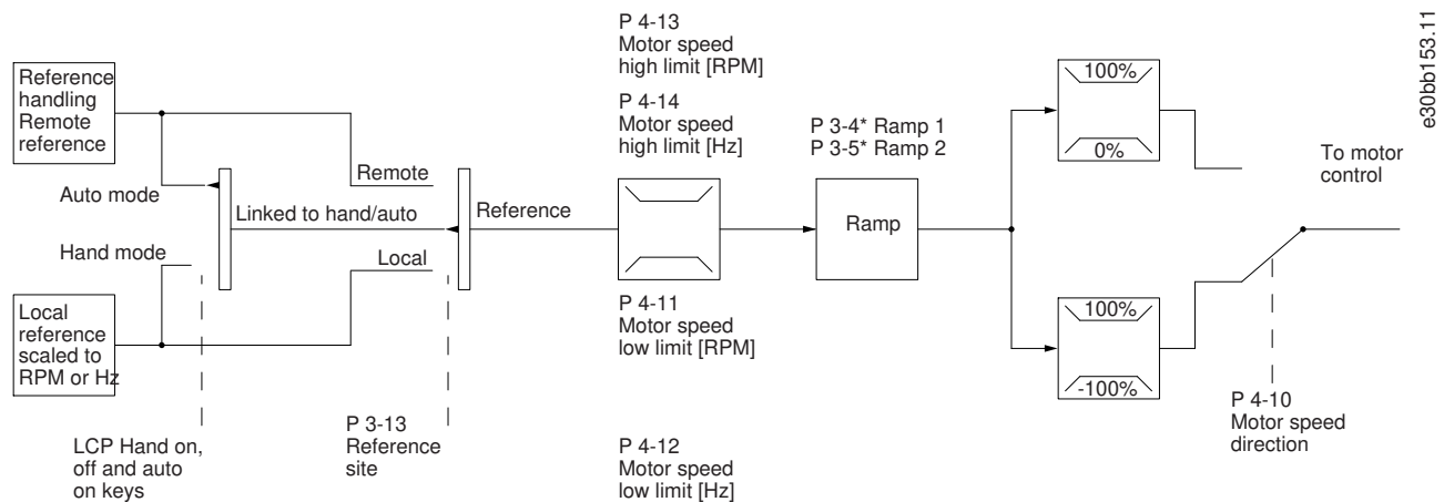
Illustration 92: Open-loop Structure
