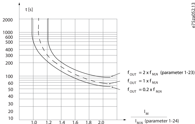
Illustration 73: ETR Characteristics
