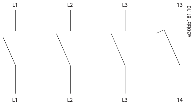
Illustration 72: Terminal Connections for C1 and C2
