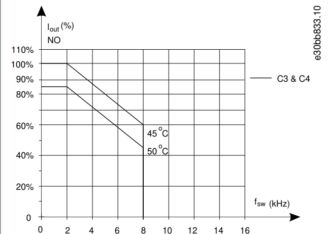
Illustration 55: Derating of I_{out} for Different T_{AMB,MAX} for Enclosures Sizes C3 and C4, using SFAVM
