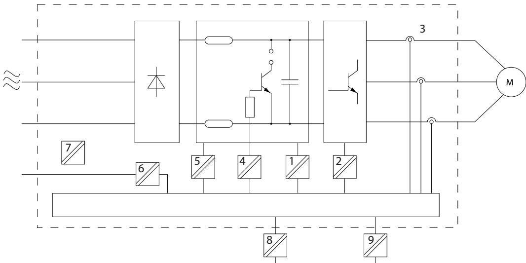
Illustration 81: Galvanic Isolation
