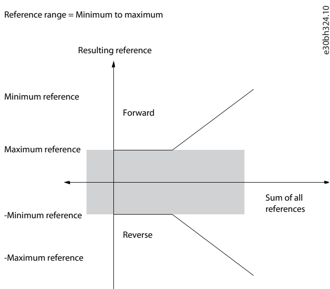
Illustration 88: Sum of All References When Reference Range is Set to 0
