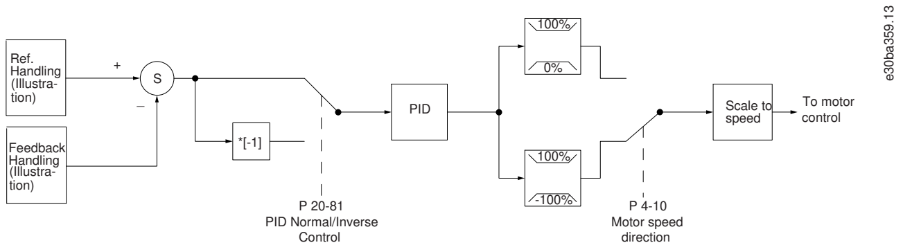
Illustration 93: Control Structure Closed-loop
