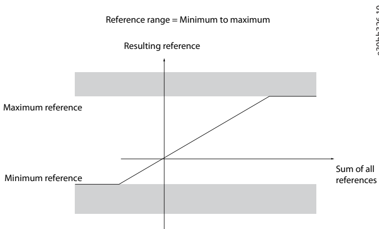
Illustration 90: Sum of all References when Configuration Mode is set to Process
